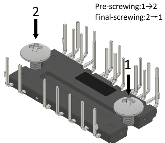
Figure13. Screwing Order
