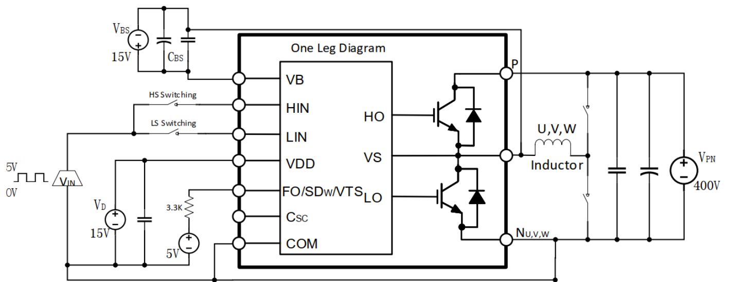
Figure4. Switching Test Circuit
