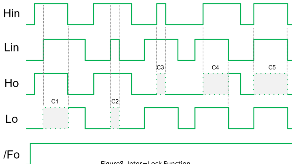
Figure8. Inter-Lock Function
